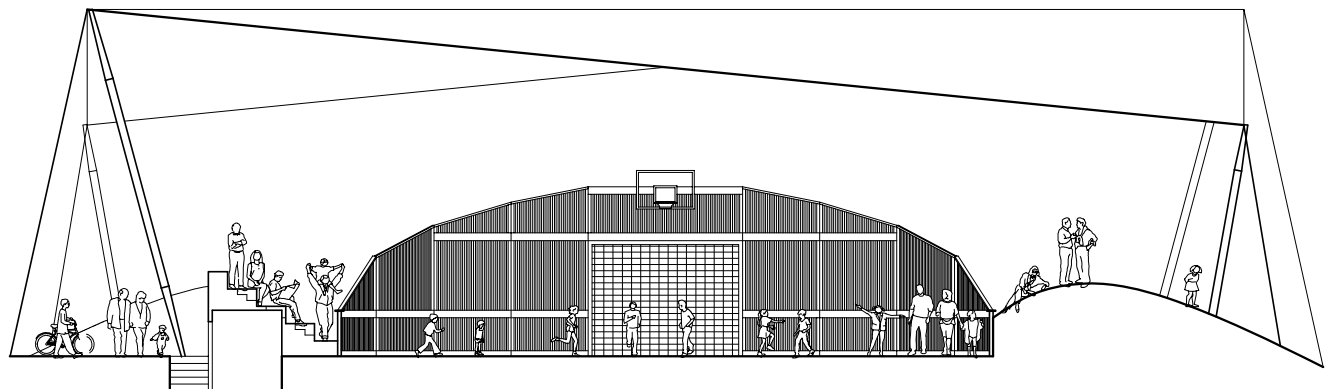
section through the homeground showing the enclosure, canopy and seating
